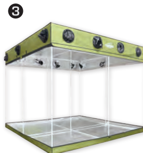
Drape the roof skin (M) over the top of the frame
